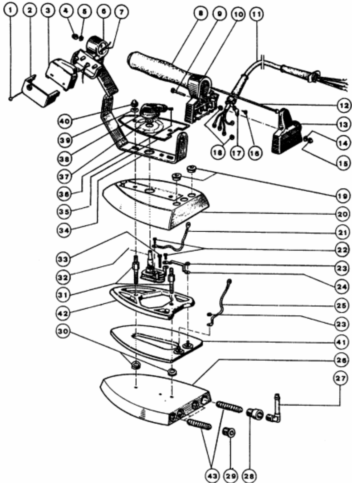
ACA115 Steam-Electric Iron
