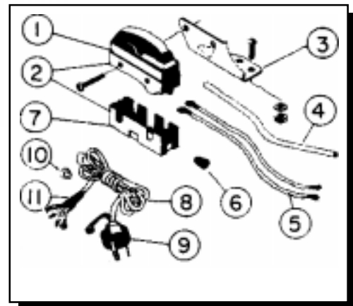
Model XB Thumb Switch Parts
